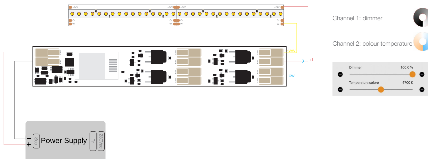
Wiring diagram: tunable White
