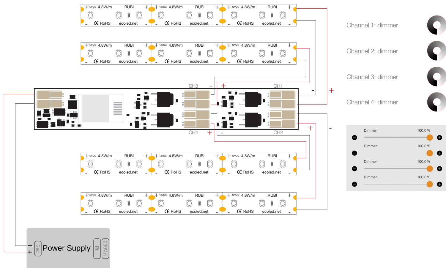
Wiring diagram: 1-2-3-4 separate channels
